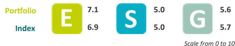
Scores Distribution 2
